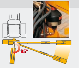
Hydraulic break-back with accumulator controlled autoreset facility
