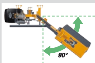
Hydraulic breakaway on power slew ram with max. relief valve (safeguards arm in case of obstacles)
